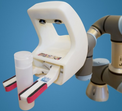
Versatile gripper with tactile sensors
